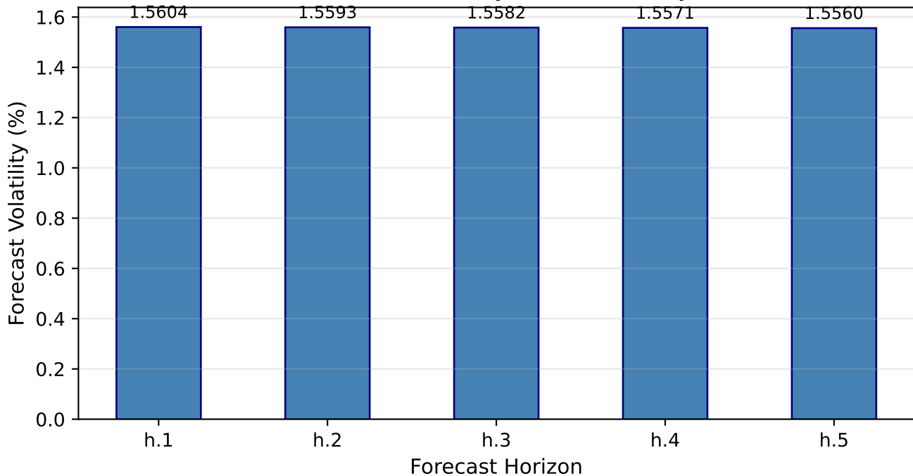
NVDA GARCH(1,1) — 5-Day Ahead Volatility Forecast
